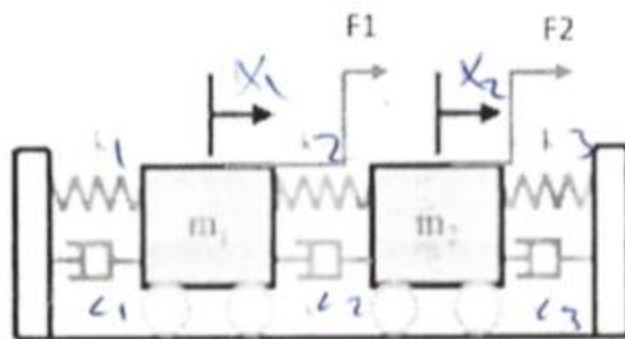
2 DOF system
